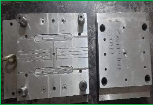
10 impression family injection mould set for LED Strips
