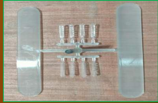
10 impression family injection mould set for LED Strips
