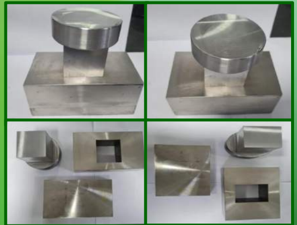
Square Die for Steel Specimen
