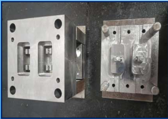
Product Name: 2 Impression Compression Mould for BHEL terminal Block Centre: Bhopal
